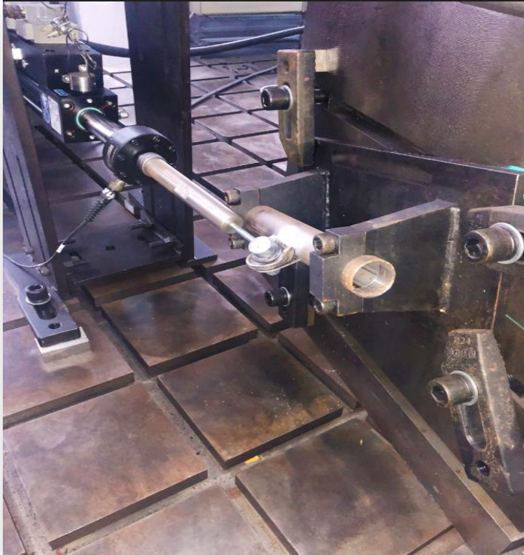
Welding Testing MTS Suspension Performance Test
